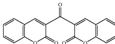
Chemical formula 1
